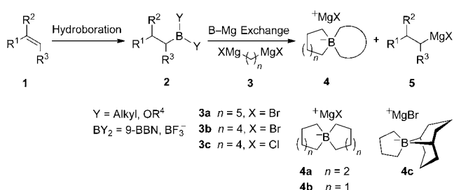
Scheme 1. Access to alkylmagnesium reagents from olefins through hydroboration and boron–magnesium exchange.
